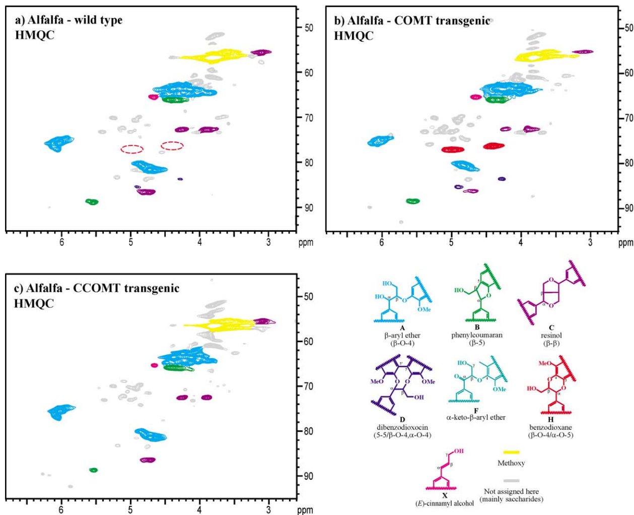
Fig. 3. Partial 2D ^{13}\text{C} – ^1\text{H} correlative HMQC NMR spectra of lignins from (a) the wild-type (b) the COMT-deficient and (c) the CCoAOMT-deficient transgenic alfalfa. The major structural units ( A–D , X and novel H ) and color-coded chemical structures are present. Dashed ovals in (a) delineate the areas in which benzodioxane units H would correlate (if they were present).
