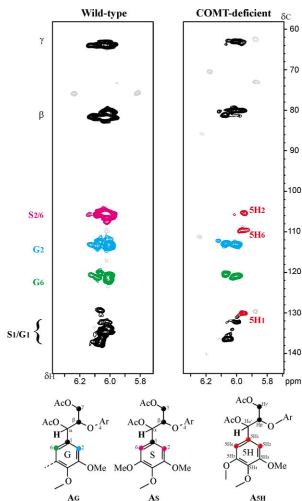
Fig. 4. Gradient-selected 2D HMBC sub-spectra showing \alpha -proton correlations in \beta -aryl ether units A (specifically with S_{2/6} , G_2 , and G_6 carbons). In the wild-type alfalfa lignin, guaiacyl ( A G ) and syringyl ( A S ) \beta -ethers are evident. In the COMT-deficient alfalfa lignin, there are only trace syringyl ( A S ) correlations, but significant new correlations from 5-hydroxyguaiacyl ( A SH ) \beta -ethers (red where distinct).
